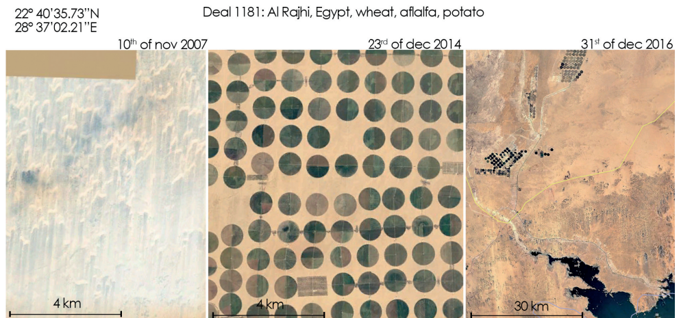
Figure 14. Example of a fully irrigated large-scale land acquisition. Images from Google Earth shows the previous land cover (desert) in 2007 to the left, and the current land use in the middle with wheat, alfalfa, potato irrigated with center pivot systems. Zooming out shows the digging of canals for irrigation purposes in the image to the right.
